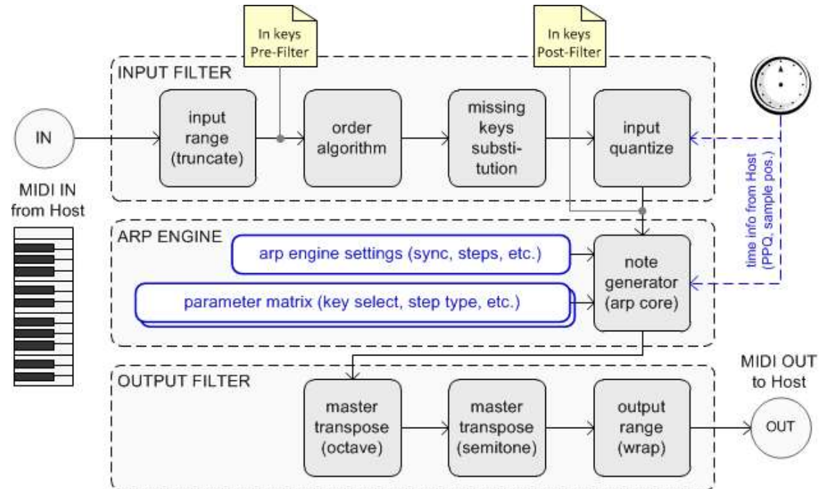
pic. 1. BlueARP processing diagram.
